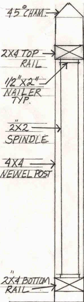
SECTION VIEW
